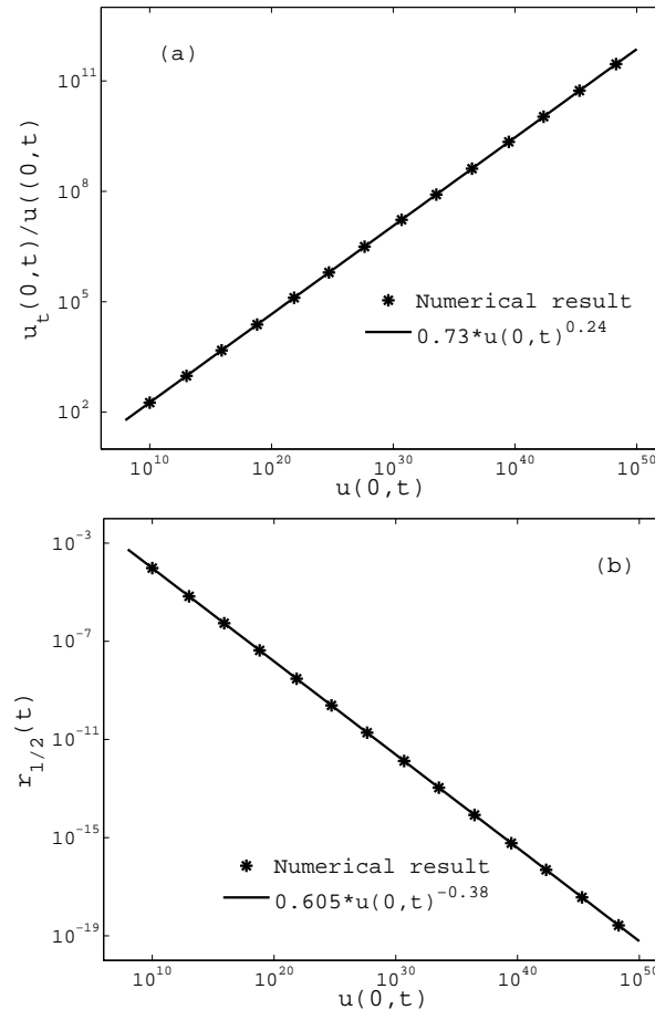
FIG. 4.1. Estimation of \alpha (\approx 1/0.24 = 4.167) and \beta (\approx 0.38/0.24 = 1.583) in dimension three by fitting.
