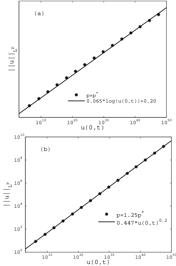
FIG. 4.3. Logarithmic blowup of \|u\|_{L^p} for p = p^* (a) and power law blow up for p > p^* (b) in dimension n = 3 . In the latter case 1/5 is exactly the theoretic predicted value 1 - p^*/p .
