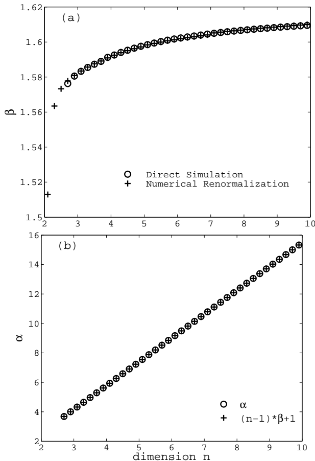
FIG. 2.3. The exponents \beta and \alpha characterizing the blowup in different spatial dimensions. In (a), because of the singularity of \nabla K and \Delta K , the exponent \beta can only be computed accurately for dimension not less than three in the direct simulation. In (b) the relation (2.5) is verified numerically for direct simulation of the blowup dynamics.
