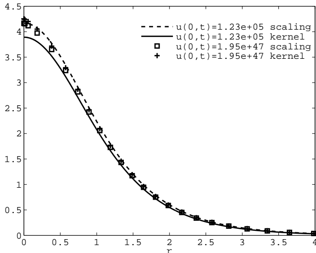
FIG. 2.2. Comparison of the two contributions \nabla \cdot (U \nabla K * U) (kernel) and \alpha U + \beta y \cdot \nabla U (scaling) in equation (2.7) for different u(0, t) in dimension three. The term \alpha U + \beta y \cdot \nabla U (dash-dots) at smaller value of u(0, t) is almost indistinguishable from both terms at larger value of u(0, t) .
