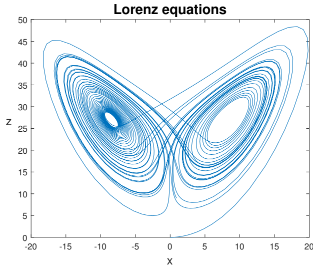
Figure 1: Numerical solution to the Lorenz ODE
