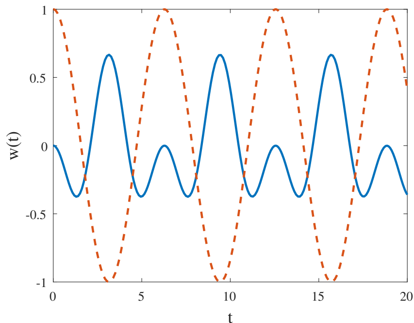
Figure 3: Numerical solution to the toy problem
