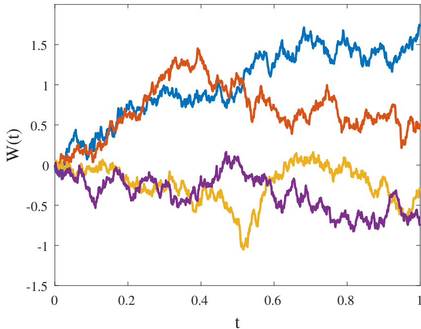
Figure 2: Different paths of Brownian motion
