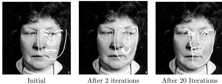
Figure 7. Search using Active Shape Model of a face, given a poor starting point. The ASM is a local method, and may fail to locate an acceptable result if initialised too far from the target
