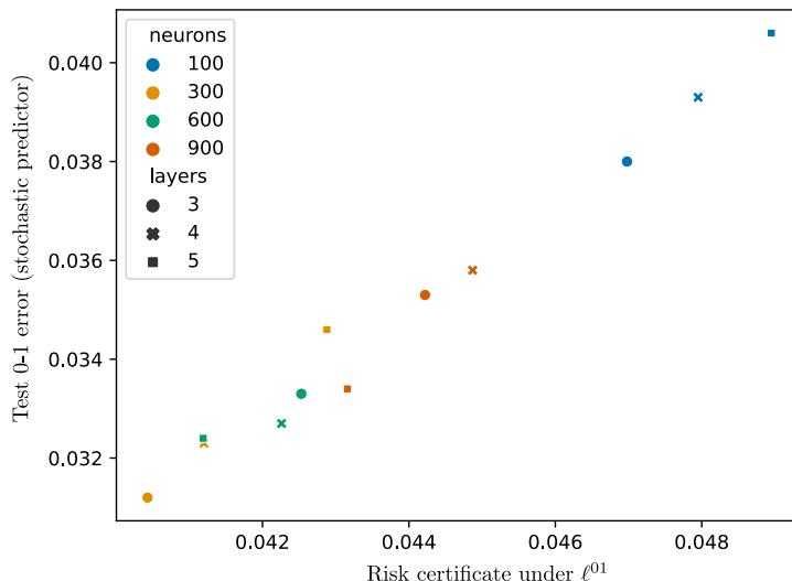
Figure 2: Risk certificate under \ell^0 vs test 0-1 error on MNIST for a set of fully connected architectures (varying the number of layers and number of neurons per layer).
