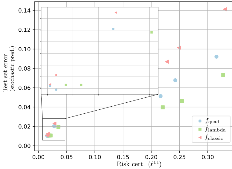
Figure 4: Scatter plot of the results obtained for MNIST using different training objectives. The x-axis shows values of the risk certificate (under \ell^{01} loss), and the y-axis shows the test set error rates, achieved by the stochastic classifier.
