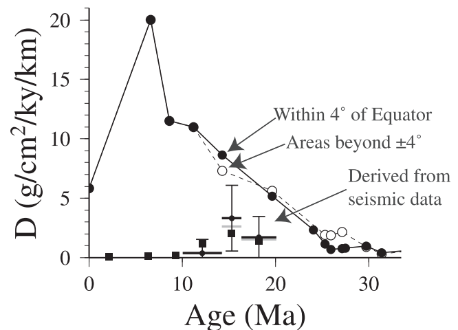
Figure 5. The graph shows the rate of change of carbonate MAR with depth below the lysocline [Heath et al. , 1977] (solid circles represent rates calculated for areas within 4^\circ of the paleoequator and open symbols are from outside the \pm 4^\circ equatorial region). Values and dates have been adjusted to the Cande and Kent [1995] timescale. The horizontal bars show estimates of dissolution rate gradients made from the Ewing seismic data using the dashed regressions in Figure 13 (the gray bars show values derived from similar regressions on basement depth differences to illustrate uncertainty). The bar horizontal extents represent the age intervals whereas the associated vertical bars represent the combined uncertainty ( 2\sigma ) in D of the regression coefficients and of the reflector ages in Table 1. The solid squares show the corresponding rates from the difference in carbonate mass between DSDP Sites 575 and 70 in Figure 12 and verify the seismic-derived results.
