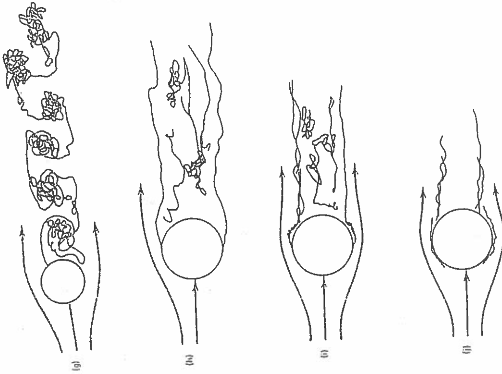
Figure 14.15 (continued) (g) 400 < Re < 10^3 , vortices turbulent at birth; (h) Re < 3 \times 10^3 , laminar boundary layer separates at 80^\circ ; (i) 3 \times 10^3 < Re < 3 \times 10^4 , separated region becomes turbulent, reattaches, and separates again at 120^\circ ; (j) 3 \times 10^4 < Re < 10^6 , turbulent boundary layer begins on front and separates on back.
