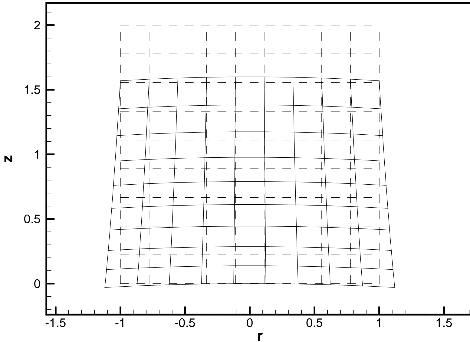
Deformation of a circular cylinder under its own weight: \nu=0.3 h=2 R=1 B=0.2
