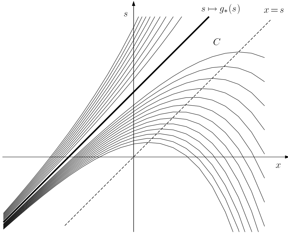
Figure 1. A computer drawing of solutions of the differential equation (3.21) in the case when \mu \equiv 0 , \sigma \equiv 1 (thus L(x) = x ) and c \equiv 1/2 . The bold line s \mapsto g_*(s) is the maximal solution which stays strictly below the diagonal in \mathbb{R}^2 . (In this particular case s \mapsto g_*(s) is a linear function.) By the maximality principle proved below, this solution is the optimal stopping boundary (the stopping time \tau_* from (3.7) is optimal for the problem (2.4)).
