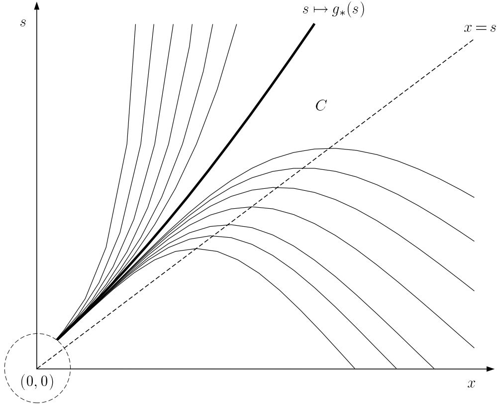
Figure 2. A computer drawing of solutions of the differential equation (3.21) in the case when X is a geometric Brownian motion from Example 4.4 below with \mu = -1 , \sigma^2 = 2 (thus \Delta = 2 ) and c = 50 . The bold line s \mapsto g_*(s) is the maximal solution which stays strictly below the diagonal in \mathbb{R}_+^2 . (In this particular case there is no closed formula for s \mapsto g_*(s) , but it is proved that s \mapsto g_*(s) satisfies (4.30).)
