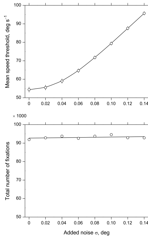
Figure 6. Effect of added noise. Optimum speed threshold v_{opt} averaged over all 140 blocks (upper panel) and corresponding total number of fixations classified by the proposed nonparametric method (lower panel) are plotted against added noise \sigma in degrees of visual angle. The continuous curves are, respectively, local and global linear regressions. For clarity, the vertical bars (upper panel) show \pm 2 SEM.
