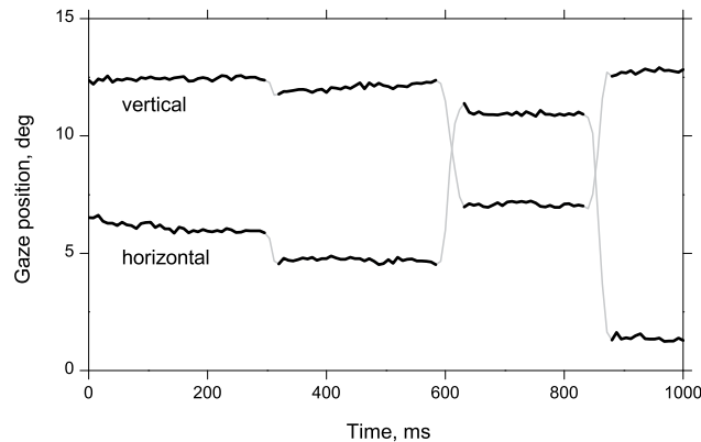
Figure 7. An example classification of a typical subsampled eye-movement trace, sampling frequency 125 Hz. Vertical and horizontal gaze positions are plotted as a function of time from the beginning of the sample. Fixations classified by the proposed nonparametric method are indicated by darker curves (compare with Fig. 5, upper panel).
