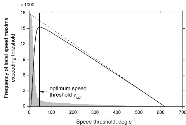
Figure 2. Distribution of local maxima in point-of-gaze speeds. The light-gray histogram shows the frequency of local speed maxima exceeding a variable threshold that ranged between the lowest and highest recorded local speed maxima (bin width \sim 2.5 \text{ deg s}^{-1} ). The dashed line shows the frequency of local speed maxima exceeding threshold under the null distribution, according to which maxima are uniformly distributed. A dotted curve traces the gap between the two, but it is largely hidden by the solid curve, which shows the loess smooth of the gap statistic (Tibshirani et al., 2001). The vertical line marks the optimum speed threshold v_{\text{opt}} . Data were based on 223 trials by one observer viewing one scene.
