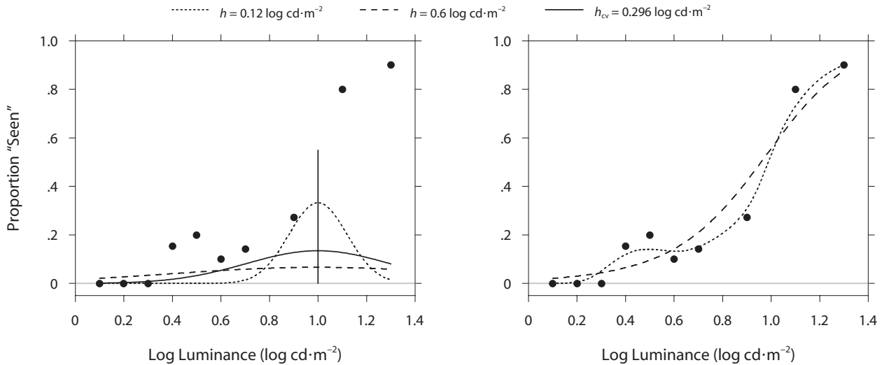
Figure 3. Effect of the weight function on a local linear estimate. The proportion of responses “seen” is plotted against log stimulus luminance. Filled circles are data from Miranda and Henson (2008), as in Figures 1 and 2. In the left panel, the dotted and dashed curves are (scaled) Gaussian weight functions with, respectively, very small and very large bandwidths h = 0.12 \log \text{cd}\cdot\text{m}^{-2} and h = 0.6 \log \text{cd}\cdot\text{m}^{-2} , centered at the point x_0 = 1.0 \log \text{cd}\cdot\text{m}^{-2} , indicated by the vertical line. In the right panel, the dotted and dashed curves are the corresponding fits obtained at x_0 , where they almost coincide, and over the rest of the stimulus range. The solid curve in the left panel shows for comparison the weight function at x_0 with the cross-validation bandwidth h_{CV} = 0.296 \log \text{cd}\cdot\text{m}^{-2} used in Figure 2.
