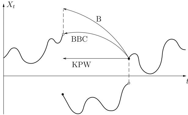
FIG. 1. The construction of three related processes from X , the stable process: “B” is the stable process conditioned to stay positive [1]; “BBC” is the censored stable process [5]; and “KPW” is the process Y in this work.
