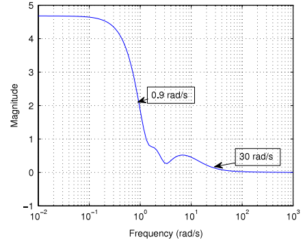
Fig. 4. Magnitude plot of T' .
