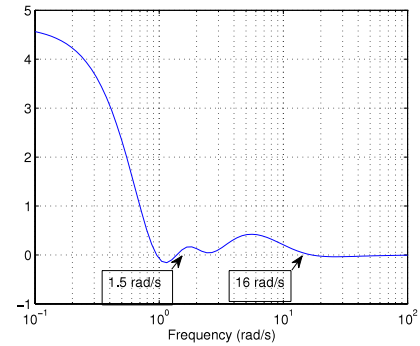
Fig. 5. \text{Re}[\bar{Z}'(j\omega)*\tilde{r}(j\omega)] vs. frequency.
