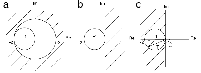
Fig. 3. Complex plane.
