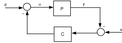
Fig. 1. Feedback interconnection of systems.
