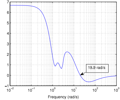
Fig. 6. |T'(j\omega)| - 2 \cos(\pi - \angle T'(j\omega)) vs. frequency.
