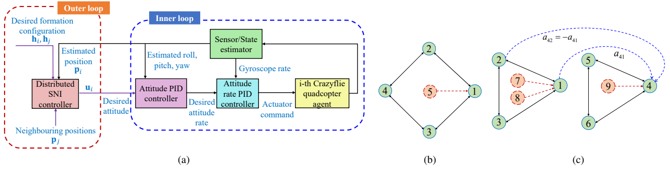
Fig. 5. (a) The proposed two-loop hardware control configuration for quadcopters to achieve time-varying group formation tracking; (b) Topology 1 connects a group of four quadcopters; (c) Topology 2 shows two subgroups, each of which contains three quadcopters. Dotted red nodes represent virtual targets.
