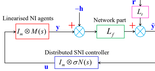
Fig. 2. An NI-based time-varying group formation tracking (TGFT) scheme for a class of multi-agent systems with multiple targets to track.
