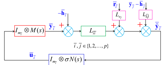
Fig. 3. The underlying formation tracking scheme for each subgroup. All such subgroups together form the complete TGFT scheme shown in Fig. 2.
