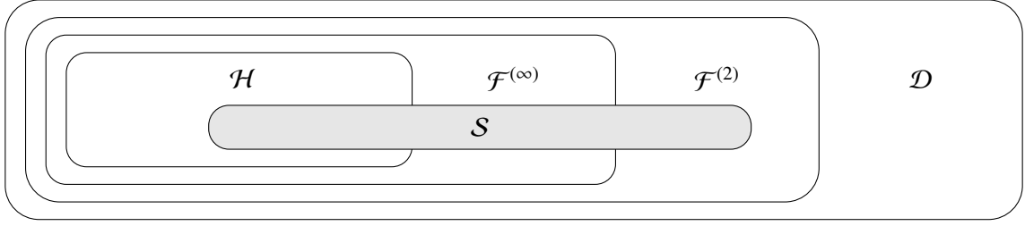
Figure 1: Venn diagram illustrating the relationships established by Lemma 3.4.
