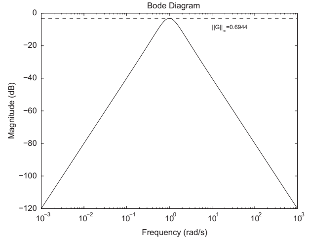
Fig. 11. The H_\infty norm of G is 0.6944.
