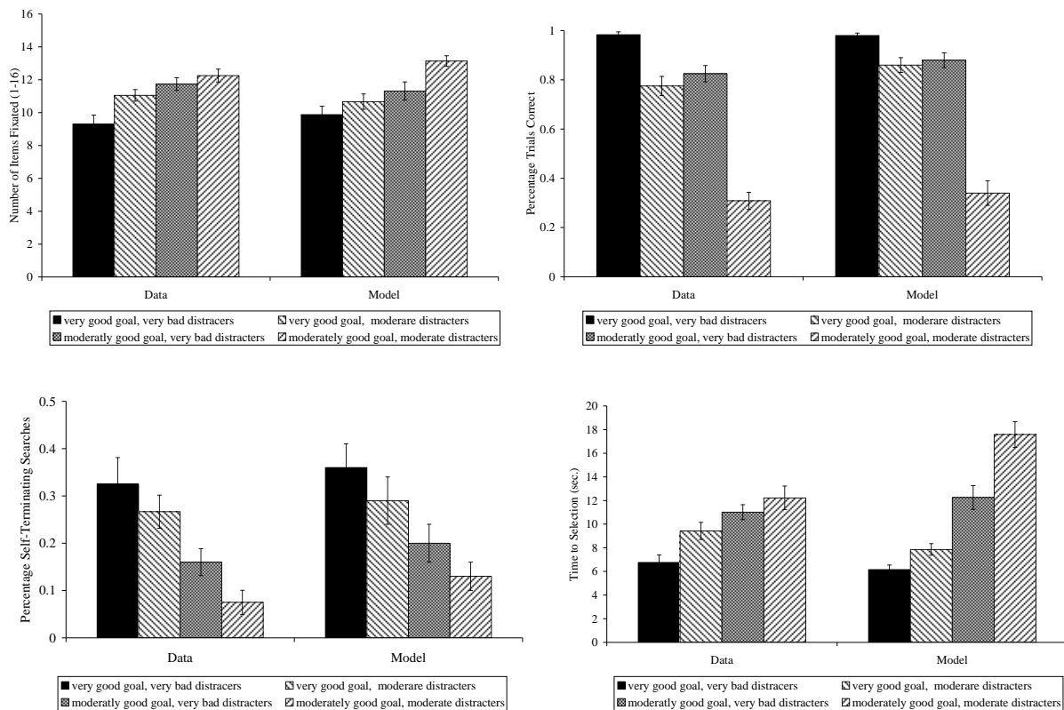
Figure 3: Data and model fits for effect of quality of goal and quality of distracter items on the (1) number of items fixated; (2) percentage of trials correct; (3) percentage of self-terminating searches; and (4) time to selection
