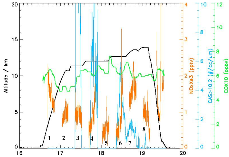
Fig. 4. Time series (in hours local time) of Egrett data on the 22 January flight: altitude (black line CO (green), NO x (orange) and particles larger than 10.2 μm (light blue line), used an indicator of in-cloud conditions, where N > 1 indicates cloud. The numbers correspond to the different transects in the flight where NO x was measured.
