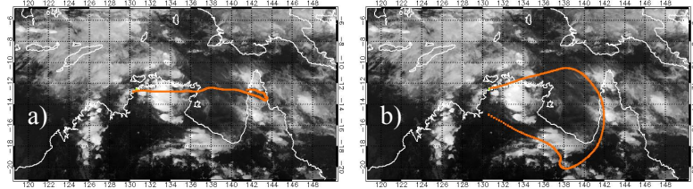
Fig. 6. 5-day backward trajectories from transects 4 (a) and 8 (b) overlaid on MTSAT IR satellite images of 22 January.
