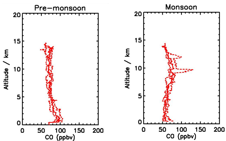
Fig. 1. Median CO vertical profile measured by the Egrett during (a) the pre-monsoon (left) and (b) monsoon (right) seasons. The dashed lines are the lower and upper quartiles of the measurements.
