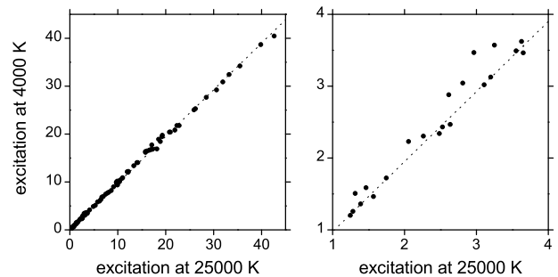
Figure 1. Modelling cone excitations by von Kries scaling. Left panel shows a linear fit with zero intercept. The right panel is an expanded section near the origin revealing local bias. Data for medium-wavelength-sensitive cones.
